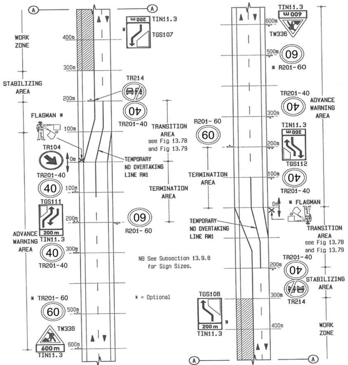
Fig. 13.49 Reduced Width Operation - 2-Way Traffic
